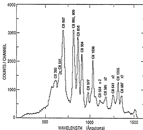
Fig. 6. VUV photon spectrum measured with a position-sensitive detector at the focal plane of a grating spectrometer located perpendicular to the incident beam direction. The xenon projectile energy was 625 MeV and the average charge state (after foil stripping just upstream of the C_{60} target) was 40+ . The peaks are labelled with identifications derived from the tabulations given in Ref. [17].
