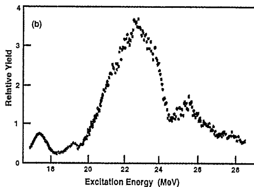
Fig. 3. Comparison of the giant dipole resonances observed in (a) the C_{60} molecule via photoionization with synchrotron radiation [9], and (b) the ^{12}\text{C} nucleus via the ^{11}\text{B}(p, \gamma)^{12}\text{C} reaction [11].
