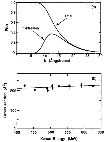
Fig. 4. (a) Calculated probabilities for the total interaction and for single-plasmon excitation as functions of the impact parameter, b , for 625 MeV ^{136}\text{Xe}^{35+} ions. (b) Calculated single-plasmon cross section (shown as a line) compared to the measured yields of \text{C}_{60}^+ from \text{C}_{60} bombarded by ^{136}\text{Xe}^{18+} ions in the energy range 420–625 MeV.
