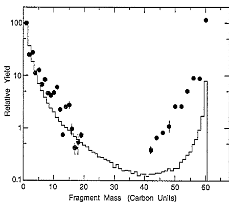
Fig. 5. Measured mass distribution (solid points) for positive fragments arising from C_{60} bombarded by 625 MeV ^{136}\text{Xe}^{35+} ions. The histogram is the distribution calculated on the basis of a multifragmentation model.
