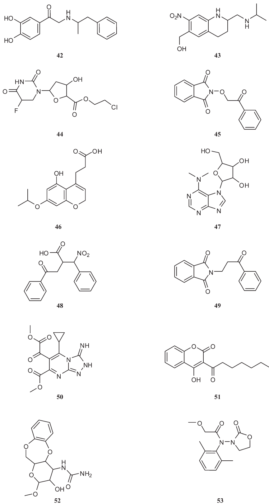
Figure 10. The chemical structures of the tested highest-ranking \beta -D-galactosidase hits (as suggested by the best QSAR models).
